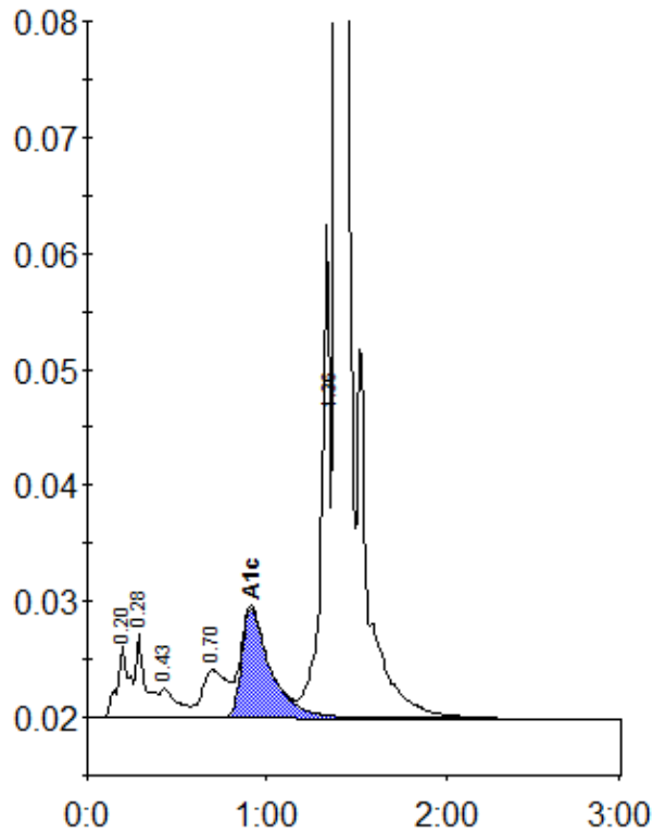
Peak table - ID: 10533252
